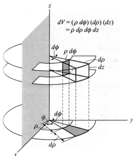
(a) Volume element in cylindrical coordinates.
